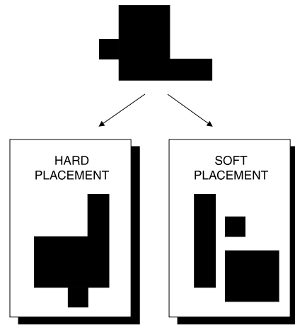
Figure 2. Macro Library
