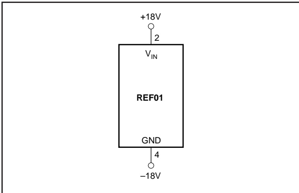
FIGURE 1. Burn-In Circuit.
